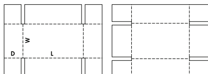
0301 Full Telescope Design Style Carton (FTD)
